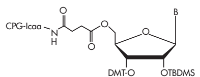
3'-DMT-2'-TBDMS-5'-CPG
