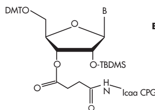
5'-DMT-2'-TBDMS-3'-CPG
