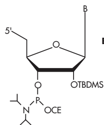
5'-DMT-2'-TBDMS-3'-Amidites
