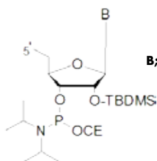
5'-DMT-2'-TBDMS-3'-Amidites
