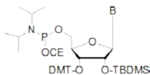
3'-DMT-2'-TBDMS-5'-Amidites
