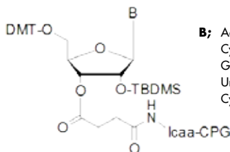
5'-DMT-2'-TBDMS-3'-CPG
